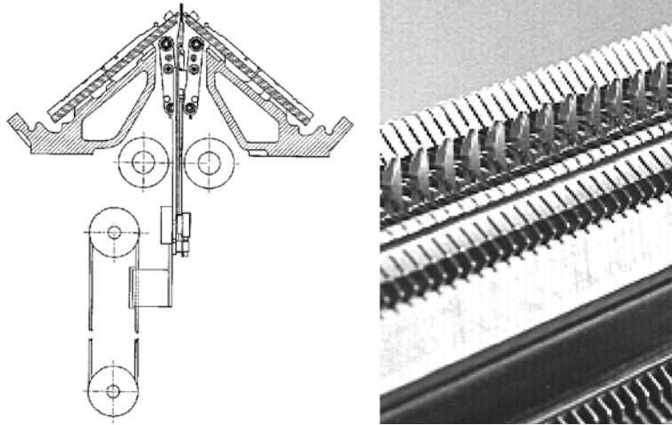
Fig. 2-29 牵拉梳
