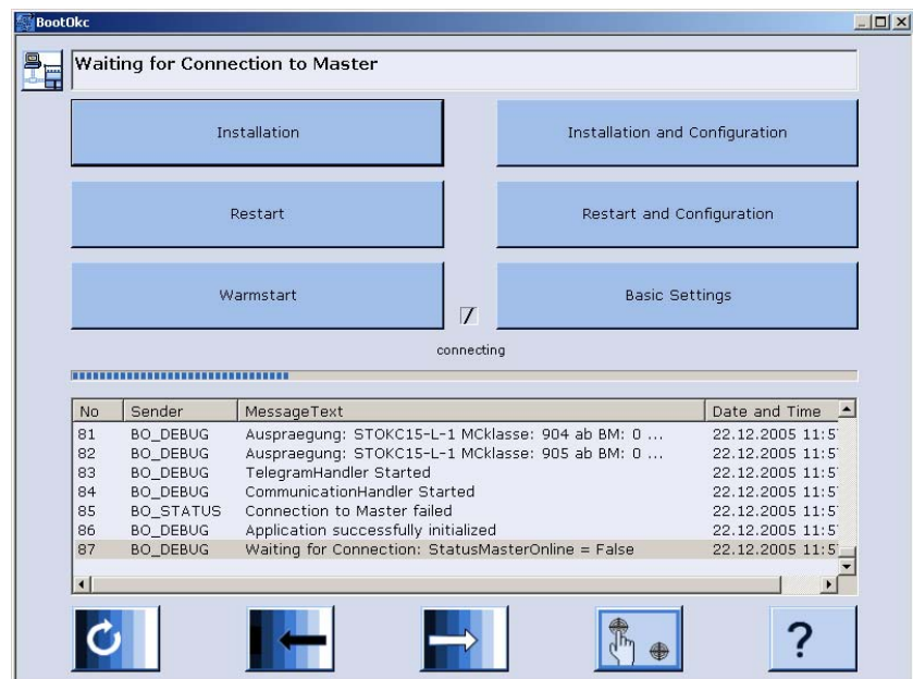
Fig. 7-23 Finestra "BootOkc"
