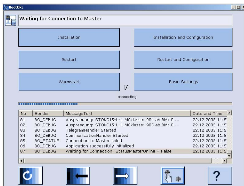
Fig. 7-22 Finestra "BootOkc"
