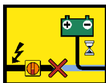
Fig. 4-41 Icona "Black-out"
