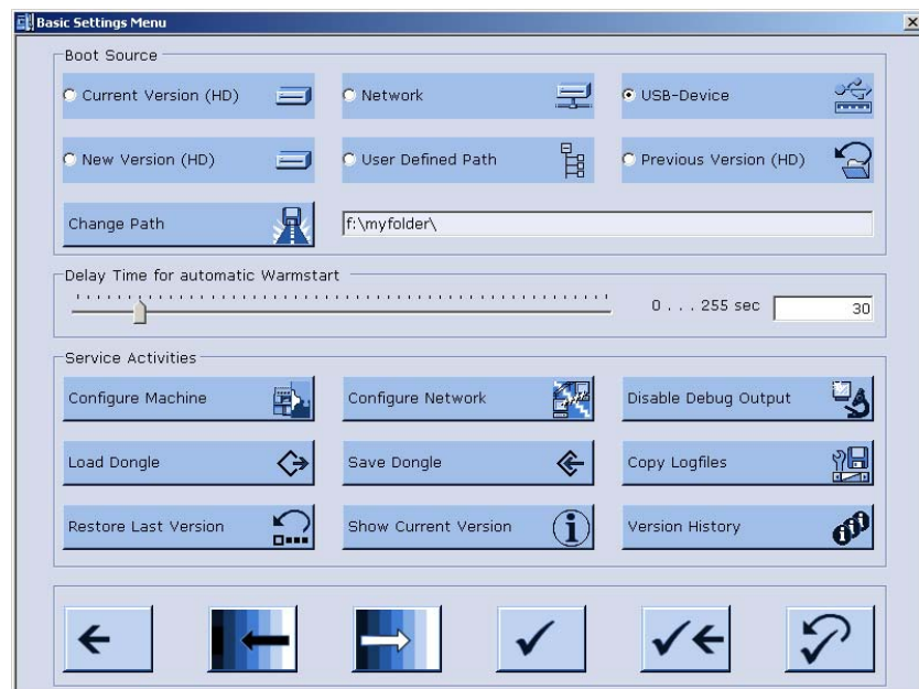
Fig. 7-6 Fenster "Basic Settings Menu"
