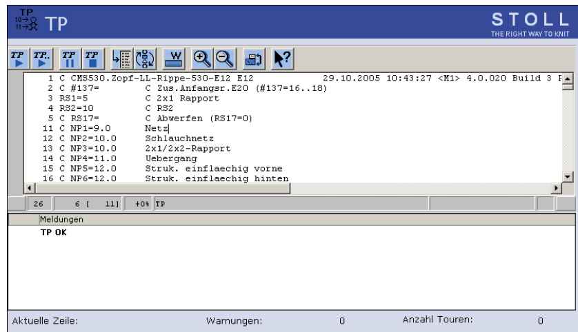
Fig. 4-95 Fenster "Programm-Test"
