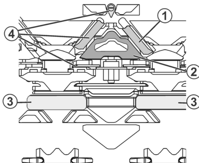
Fig. 2-17 Stricksystem
