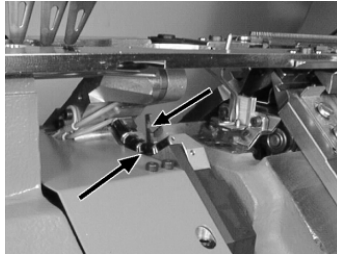
Fig. 5-19 Klemmritzel
