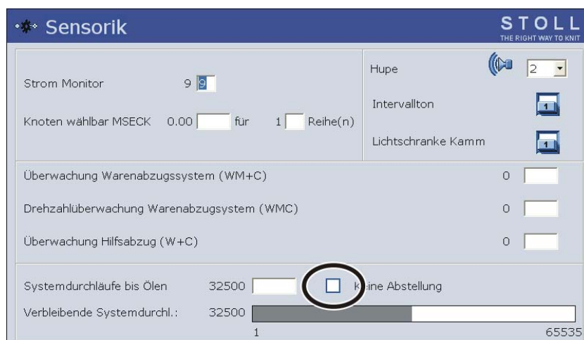
Fig. 5-36 Fenster "Sensorik"
