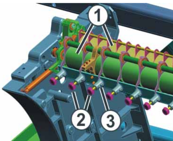
Fig. 2-33 Tirage principal
