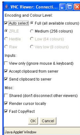
Fig. 10-10 Fenêtre "VNC Viewer: Connection Details"
