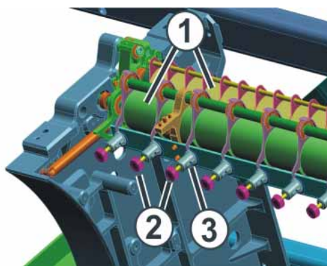
Fig. 2-28 Tirage principal
