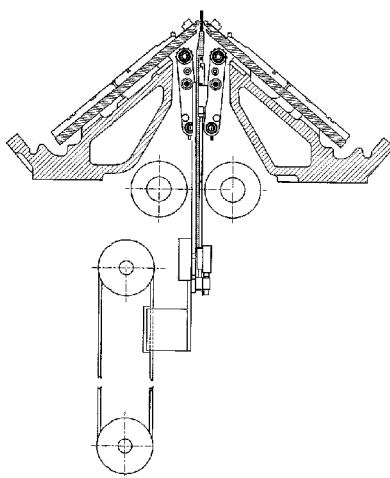
牵拉梳
