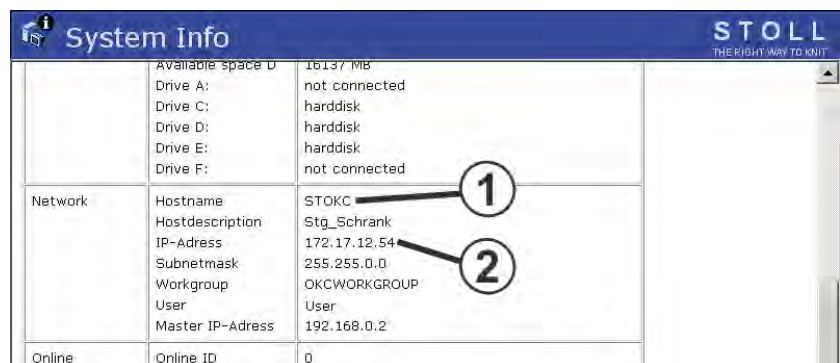
Fenster "System Info"
