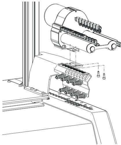
Mounting the friction feed wheel
