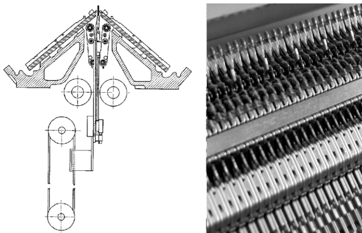
牵拉梳
