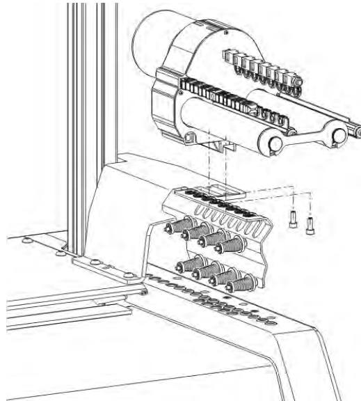
Mounting the friction feed wheel
