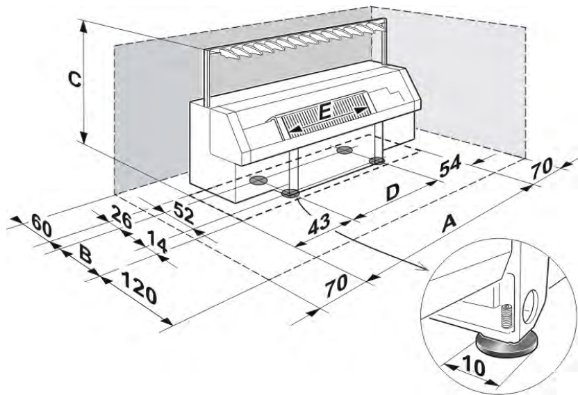
Machine dimensions (in cm)
