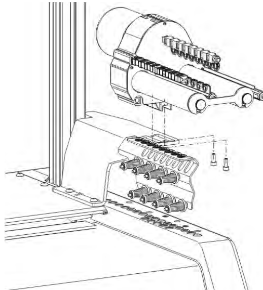
Mounting the friction feed wheel
