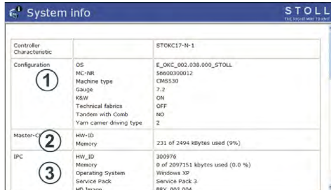
Fenster "System Info"
