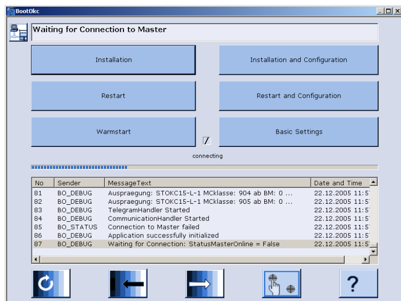
Fenster "BootOkc"
