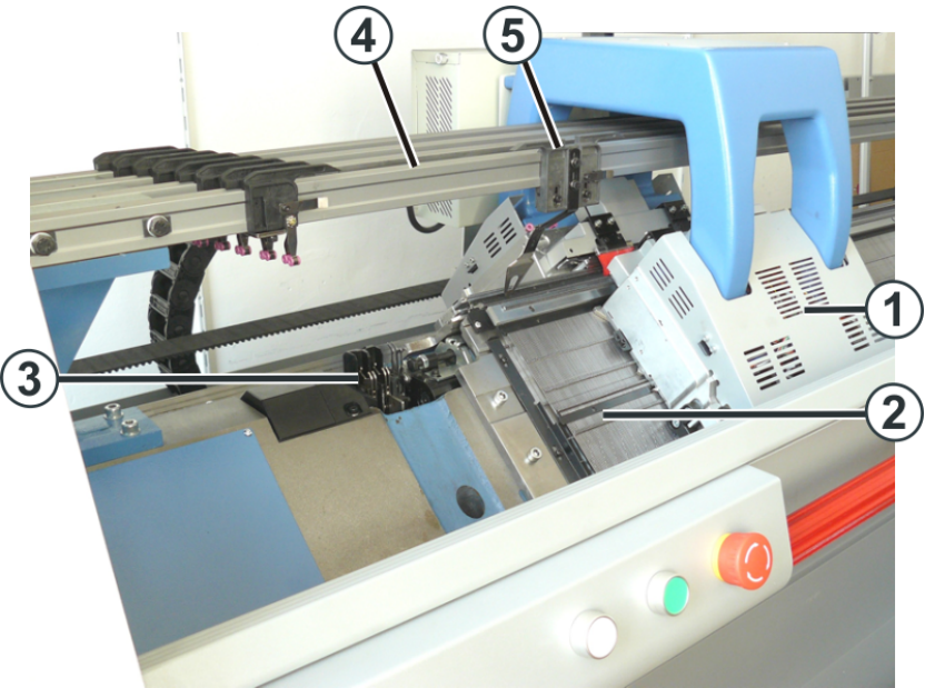
Inner view of the knitting machine
