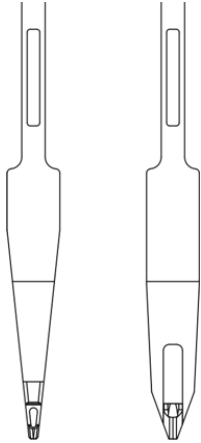
Comparison of "Narrow and standard yarn carrier tip"
